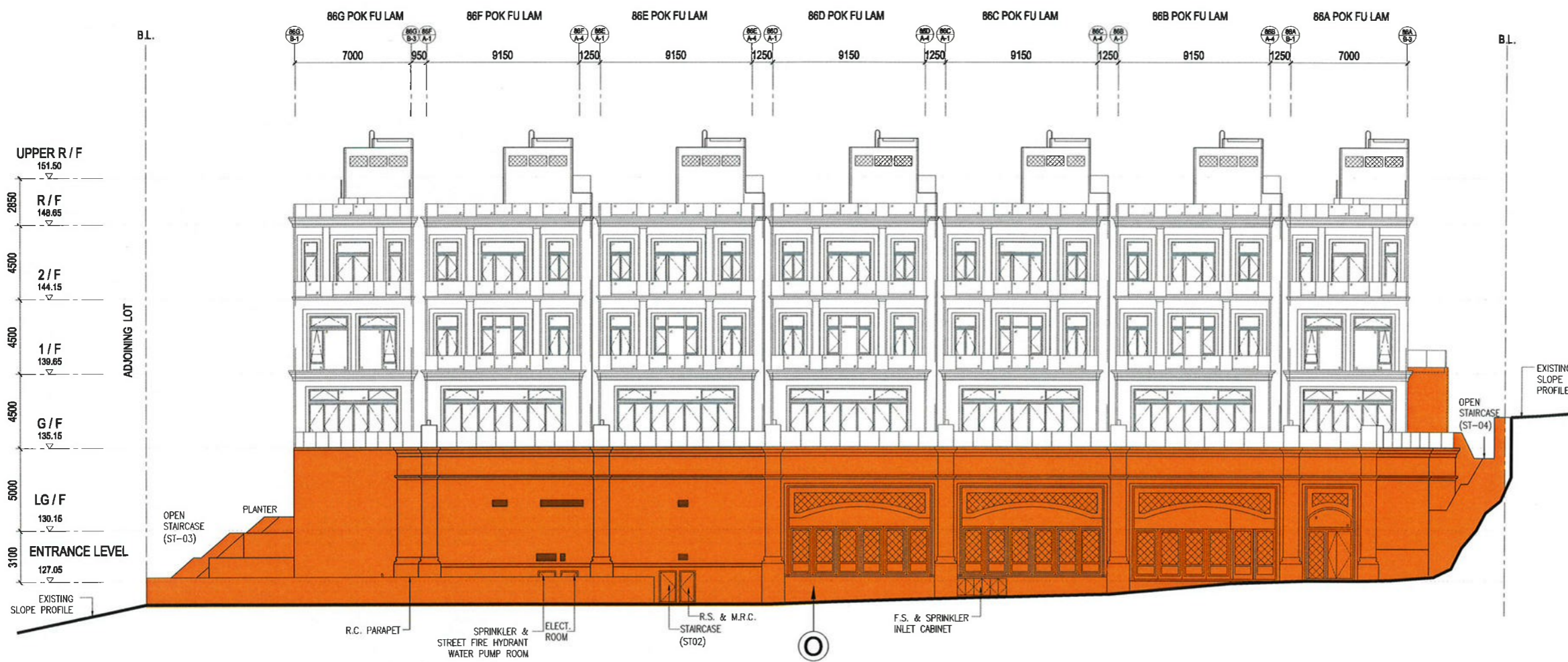
SITE ELEVATION 1
