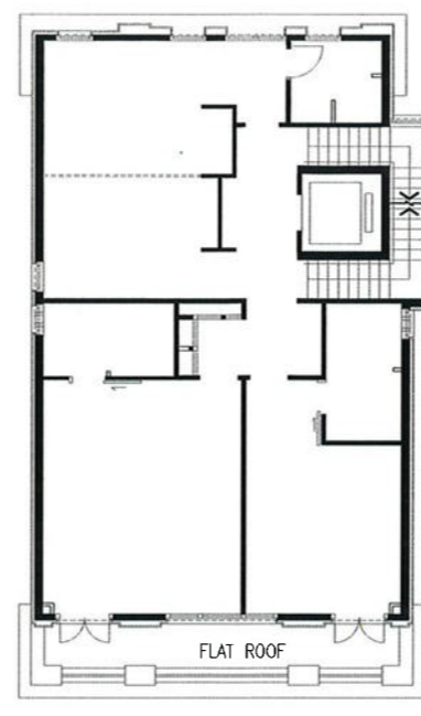
FIRST FLOOR PLAN FOR 86C POK FU LAM ROAD
