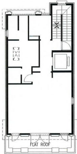
SECOND FLOOR PLAN FOR 86A&G POK FU LAM ROAD
