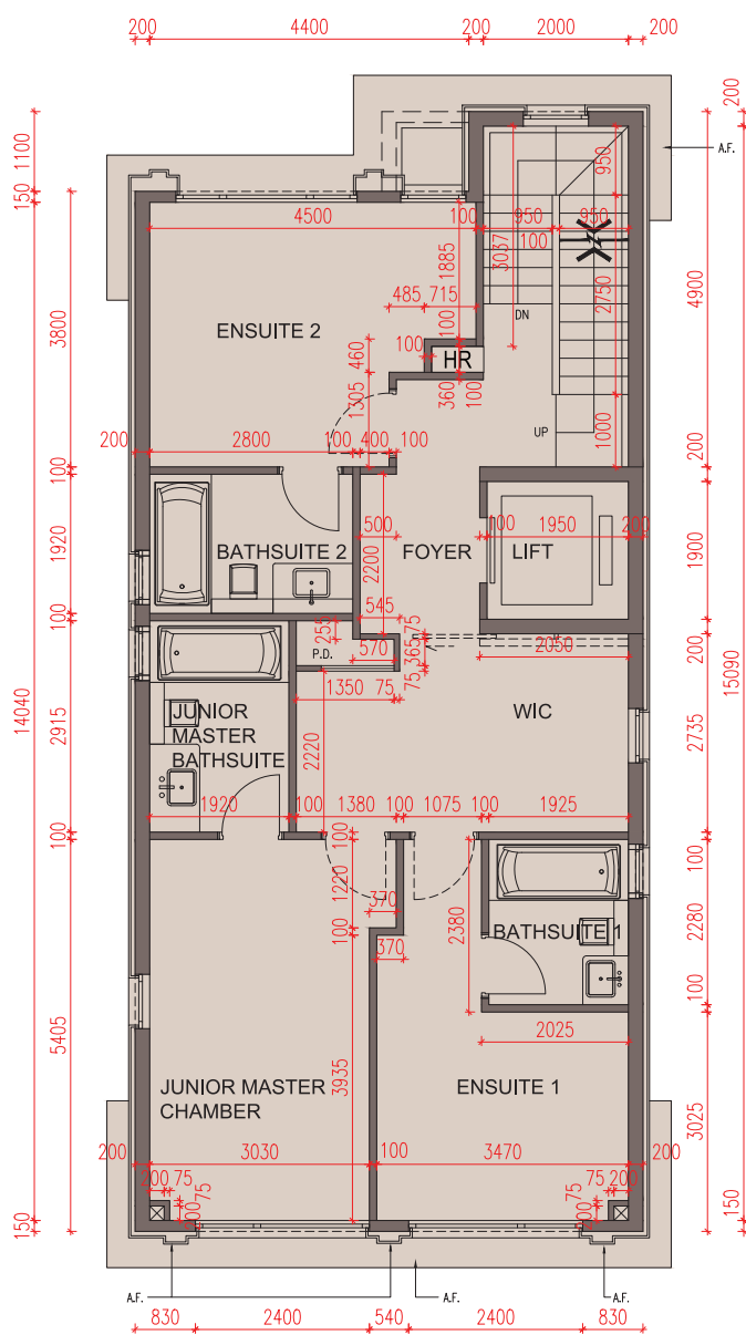
FIRST FLOOR PLAN 一樓平面圖
